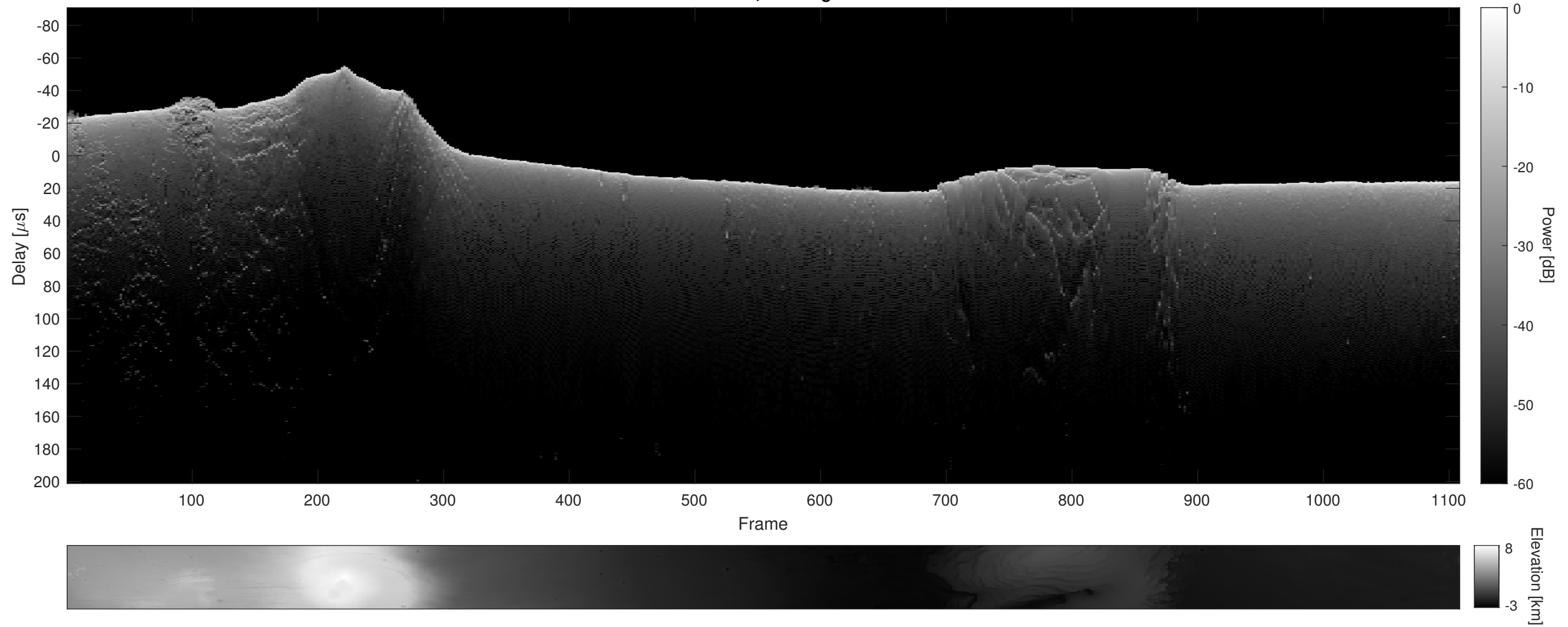
Orbit 14090, Cluttergram
