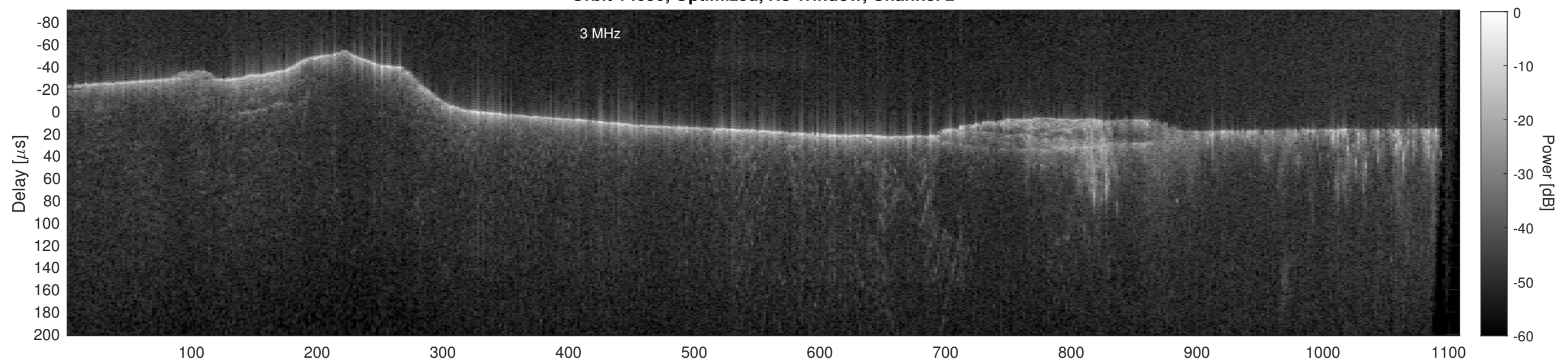
Orbit 14090, Cluttergram
