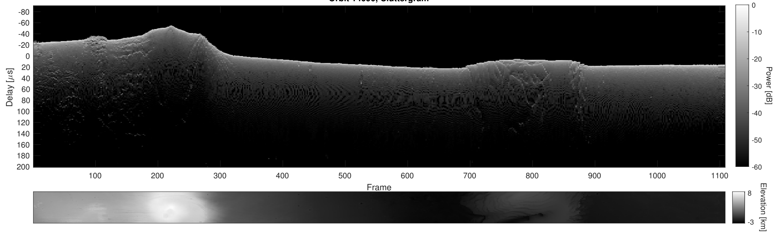
Orbit 14090, Cluttergram
