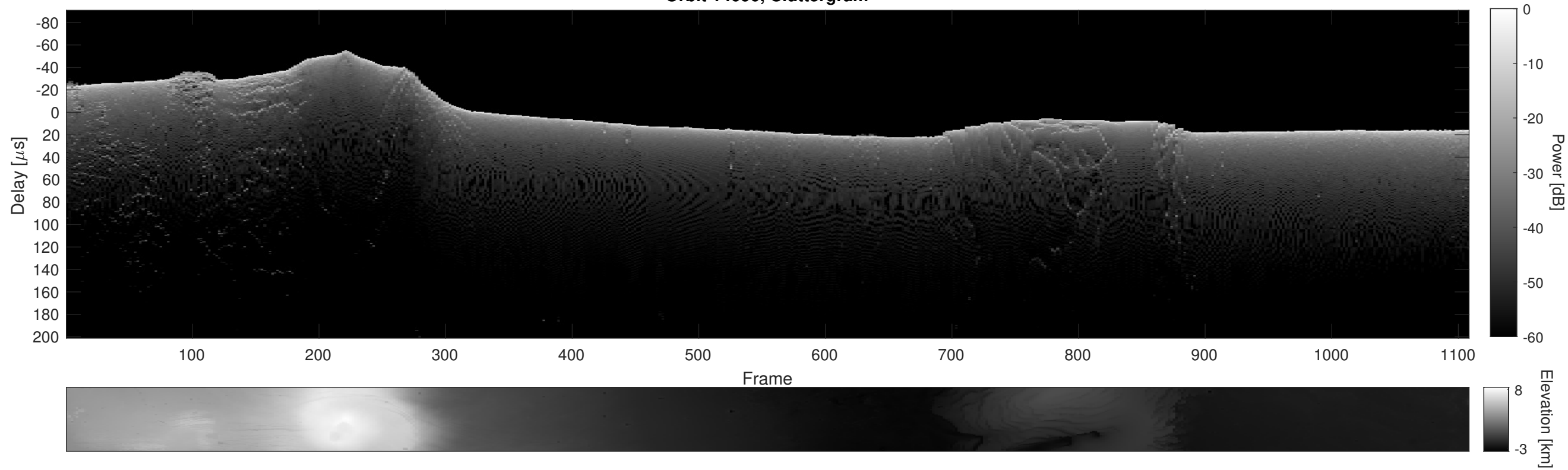
Orbit 14090, Cluttergram
