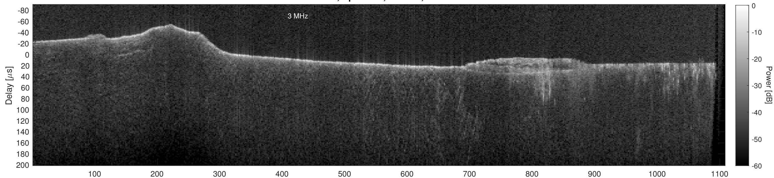
Orbit 14090, Cluttergram
