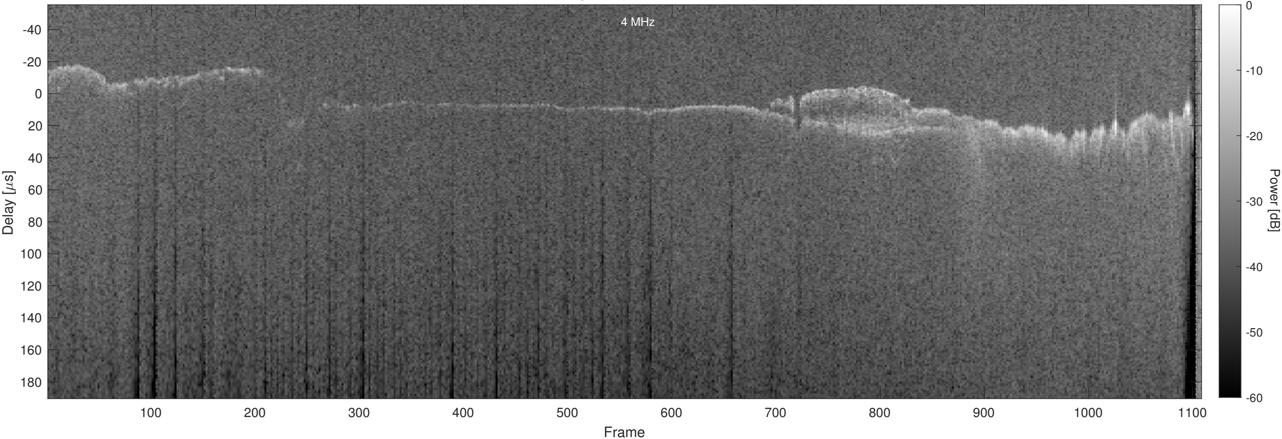
Orbit 14092, Chapman, No Window, Channel 2
