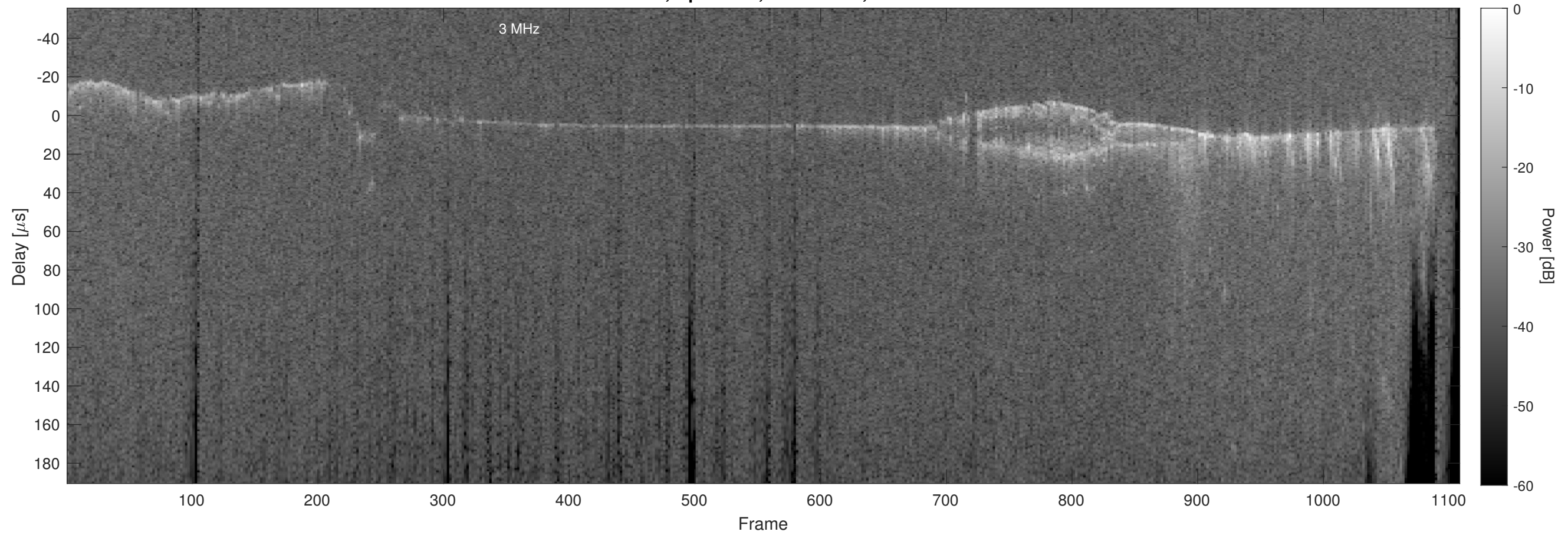
Orbit 14092, Optimized, No Window, Channel 2
