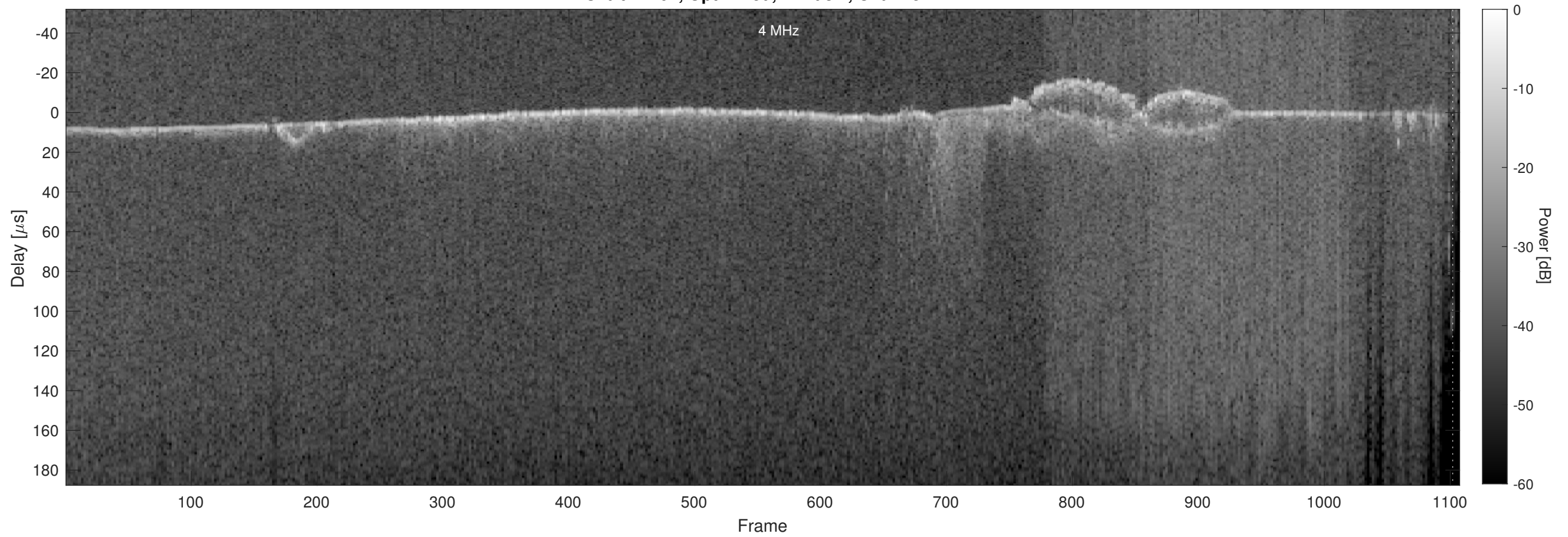
Orbit 14101, Optimized, Window, Channel 2
