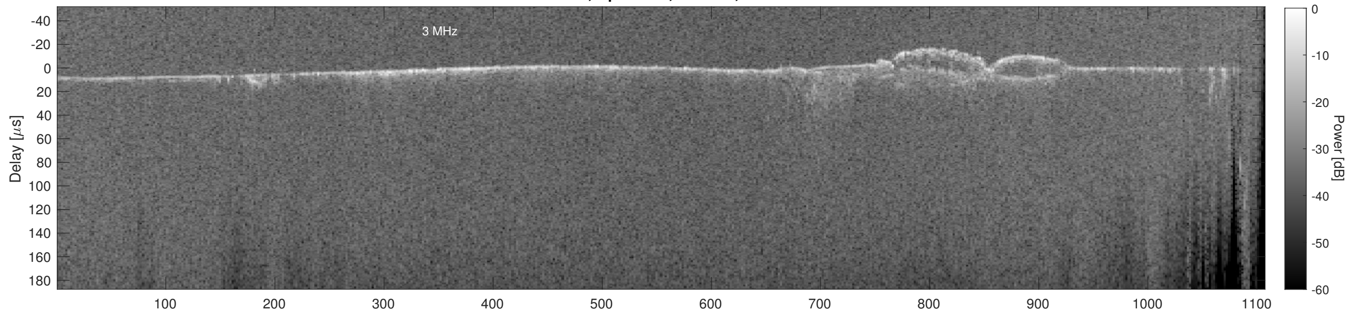
Orbit 14101, Cluttergram
