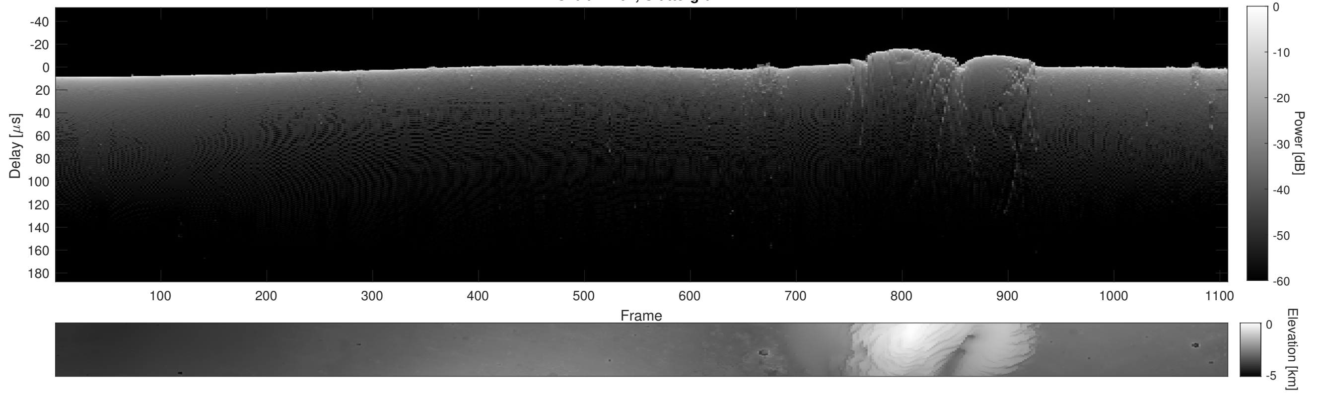
Orbit 14101, Cluttergram
