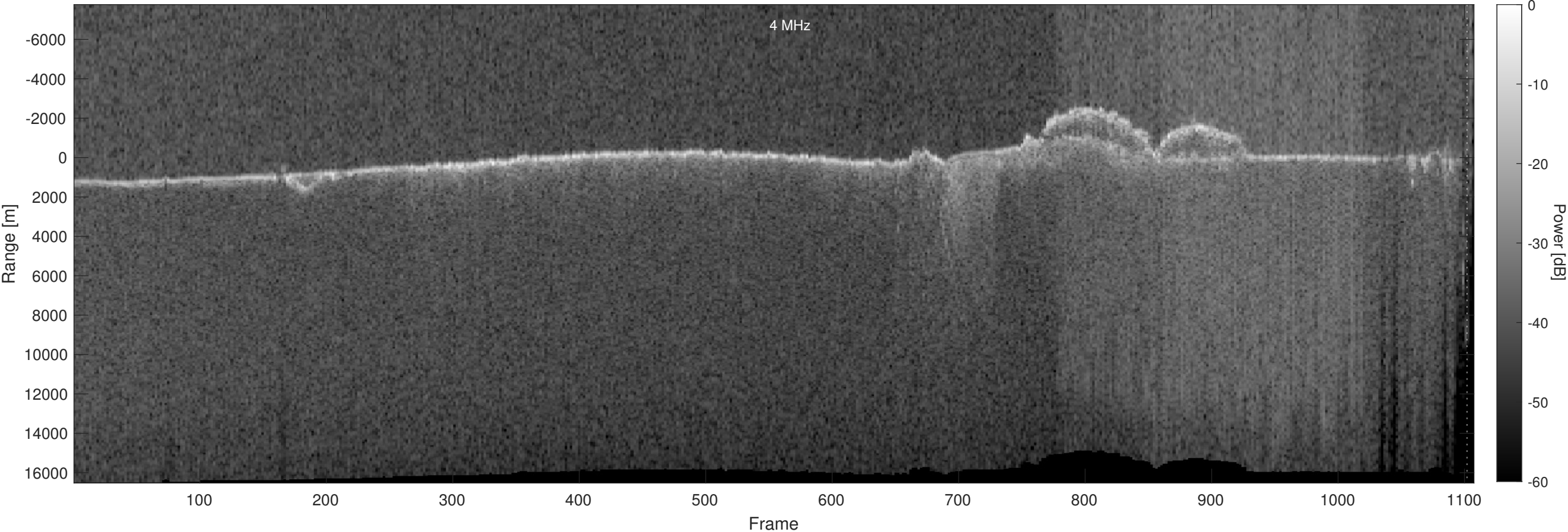
Orbit 14101, Optimized, Window, Depth-Corrected, Channel 2
