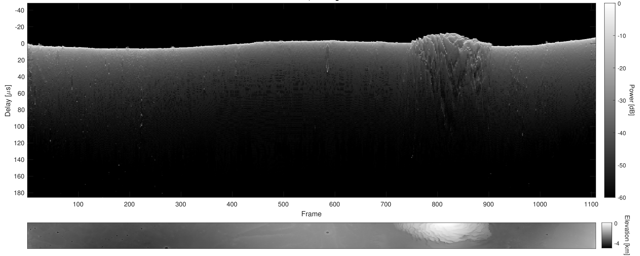
Orbit 14102, Cluttergram
