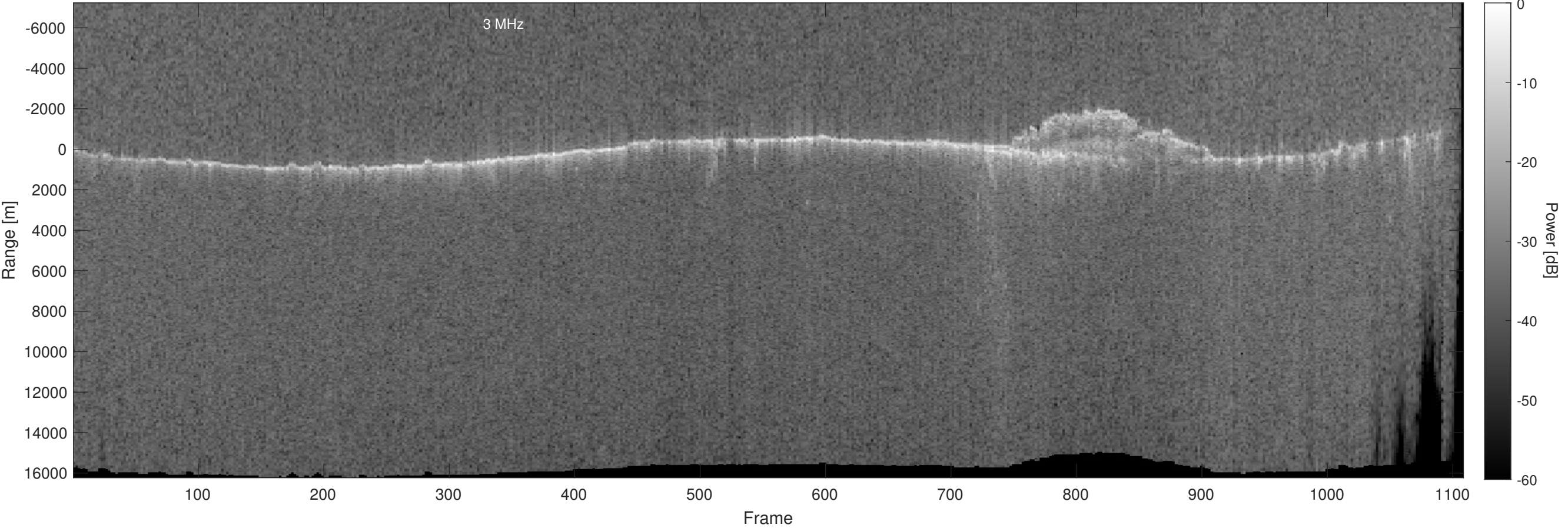
Orbit 14102, Optimized, No Window, Depth-Corrected, Channel 2
