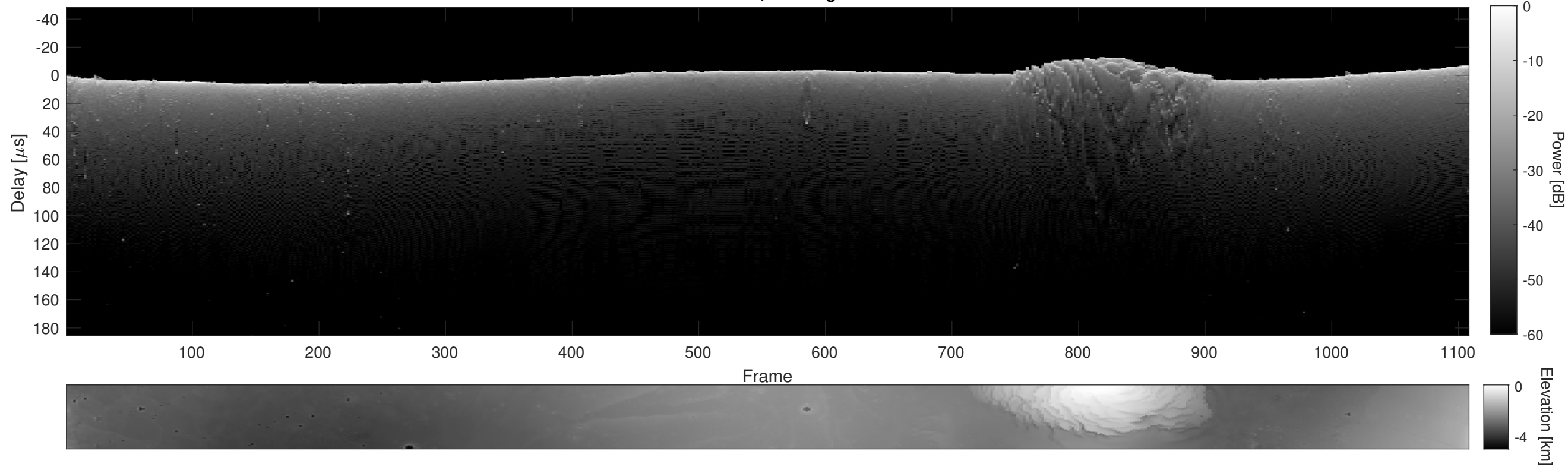
Orbit 14102, Cluttergram
