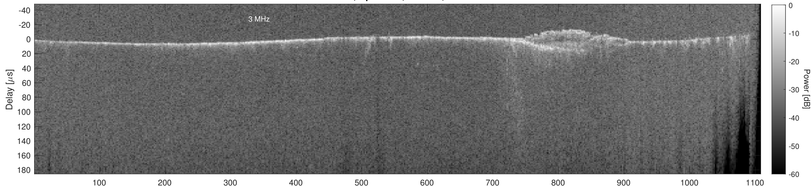
Orbit 14102, Cluttergram
