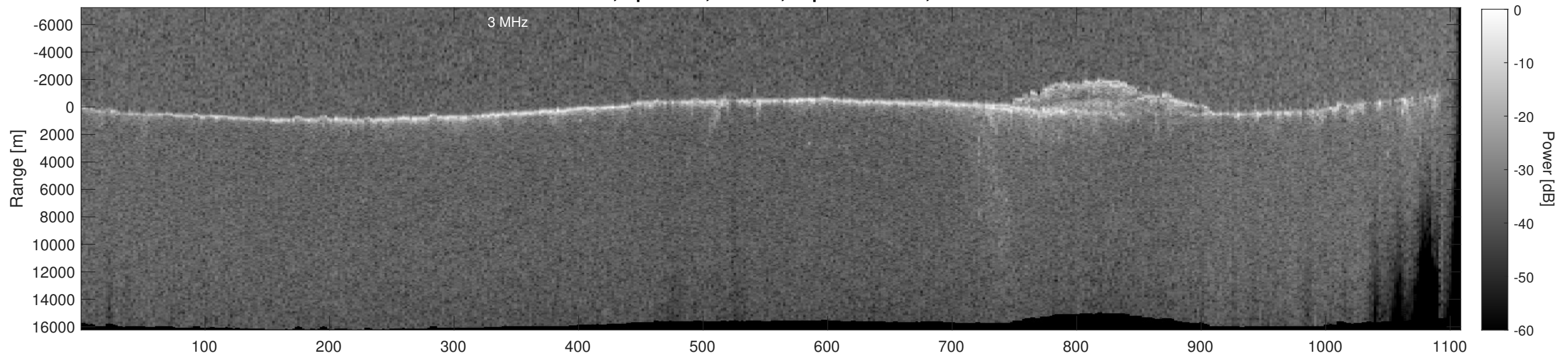
Orbit 14102, Depth-Corrected Cluttergram
