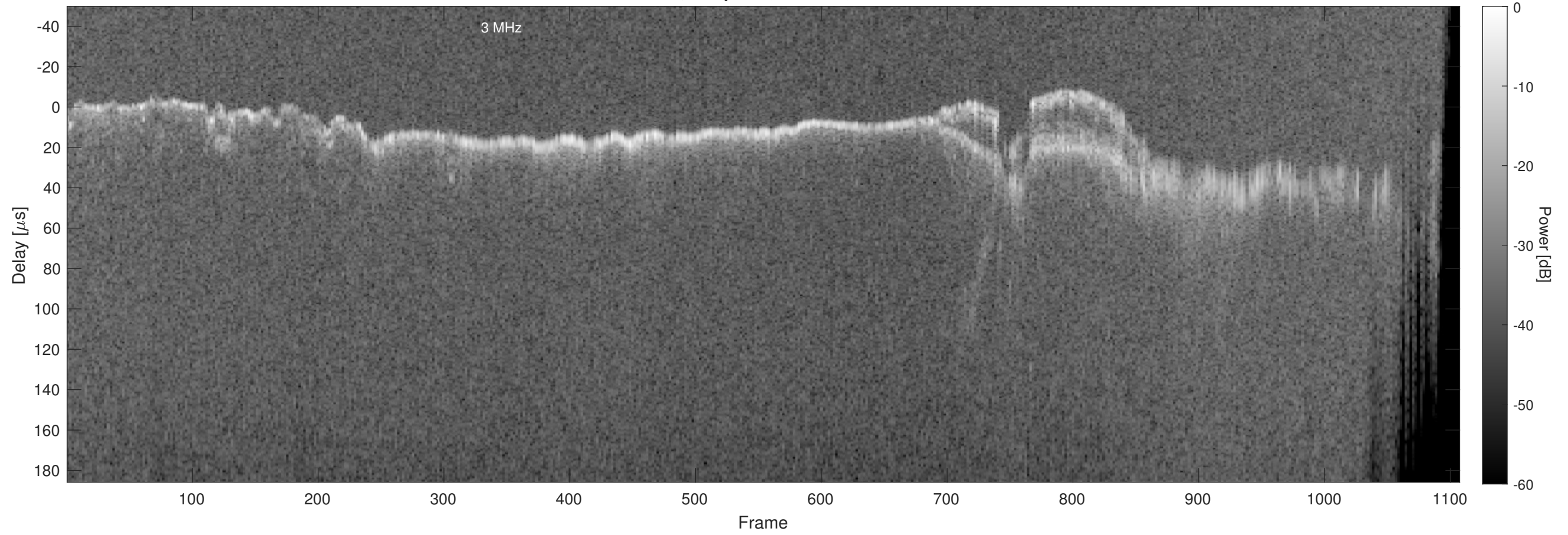
Orbit 14103, Chapman, Window, Channel 2
