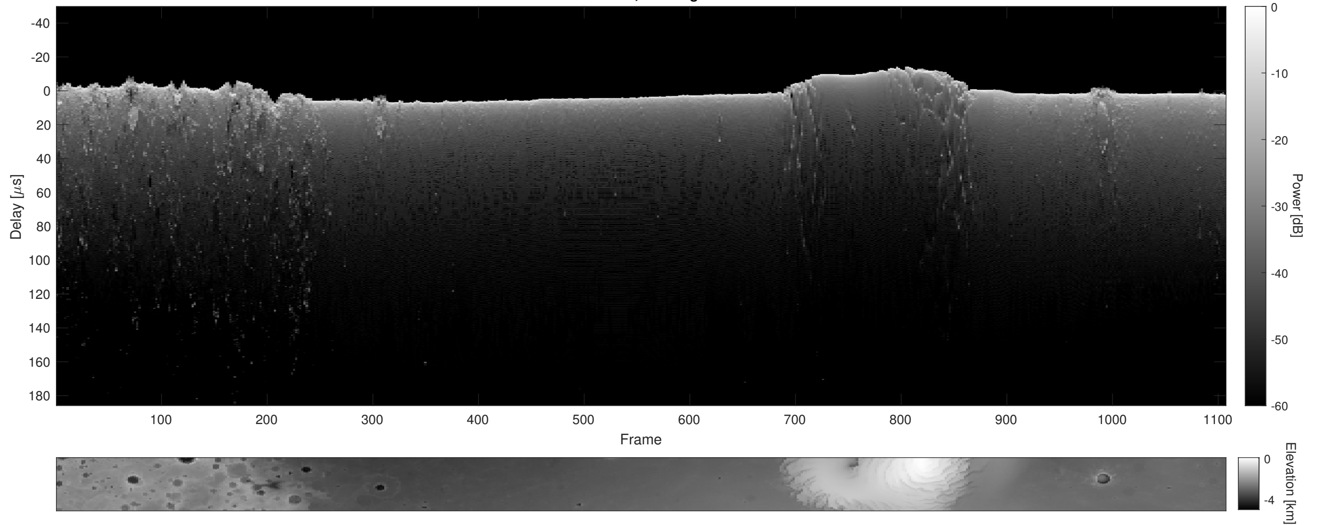
Orbit 14103, Cluttergram
