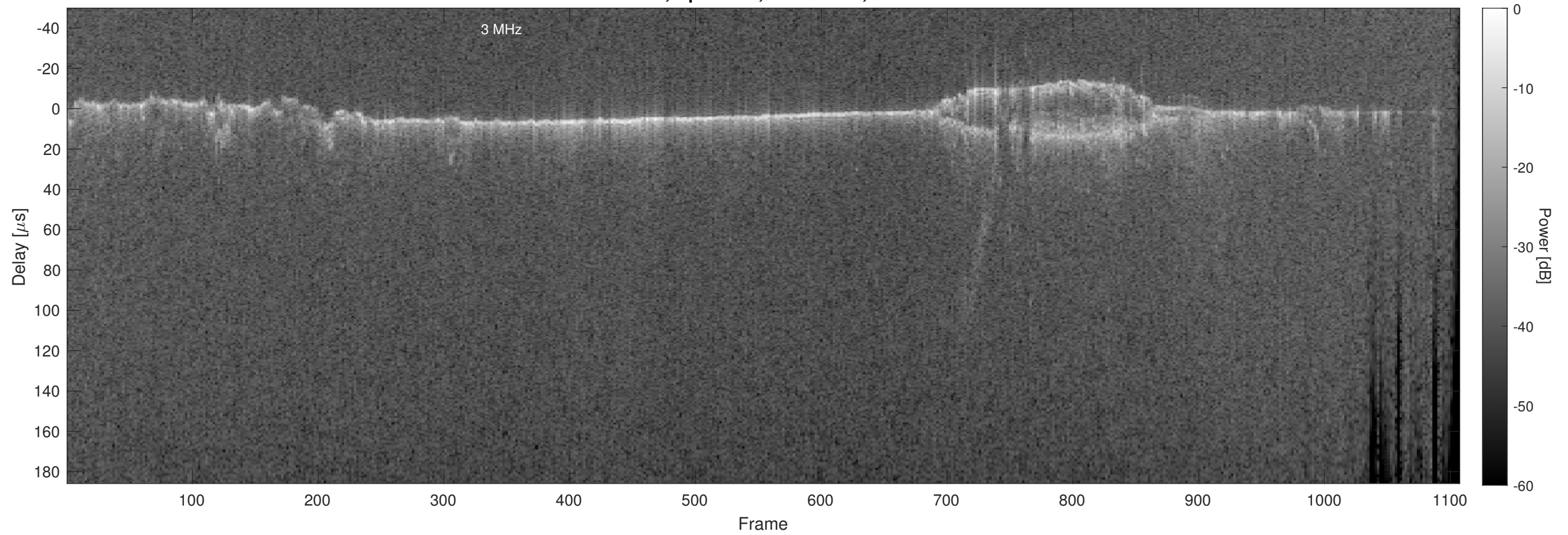
Orbit 14103, Optimized, No Window, Channel 2
