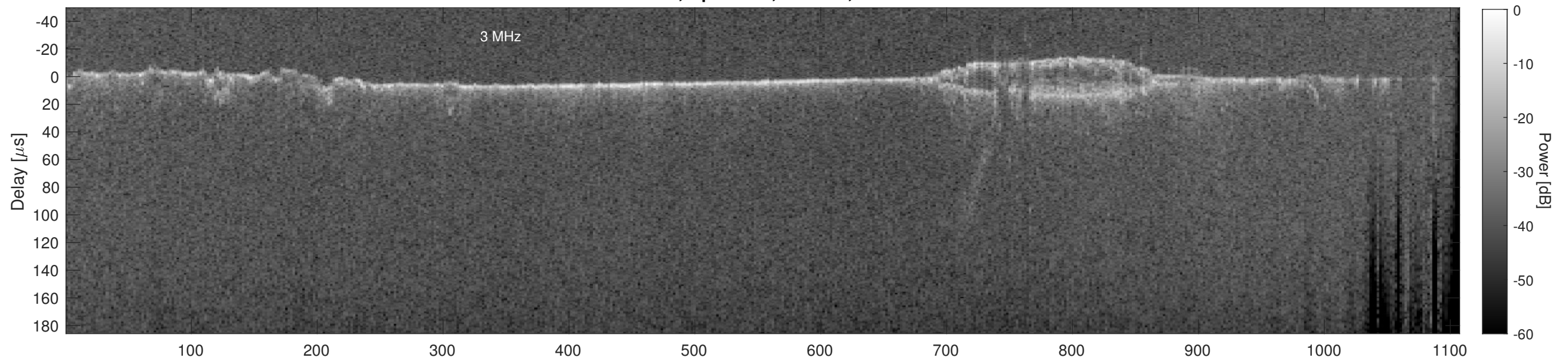
Orbit 14103, Cluttergram
