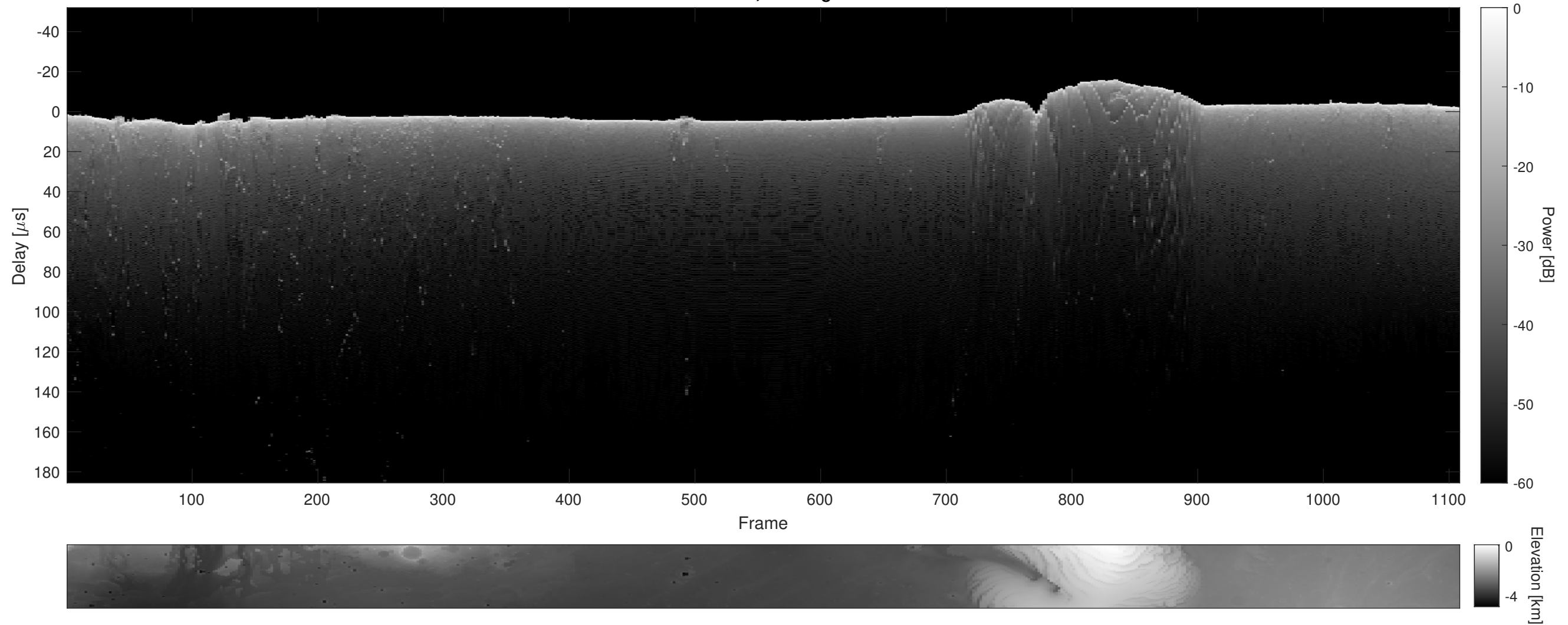
Orbit 14107, Cluttergram
