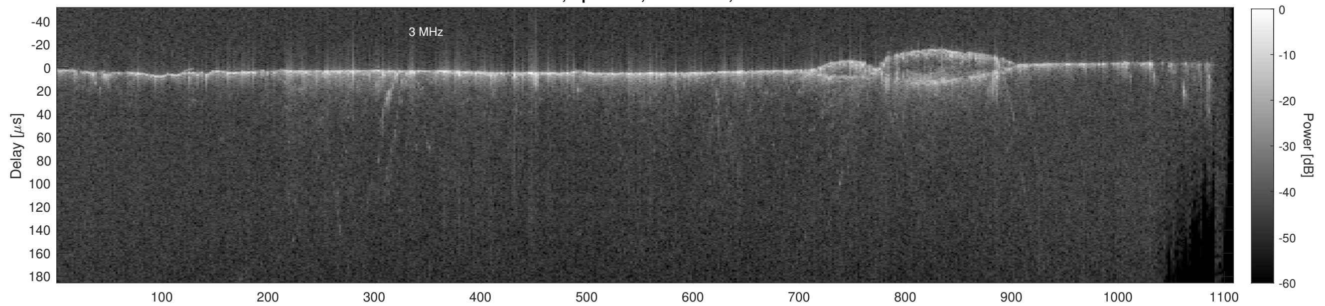
Orbit 14107, Cluttergram
