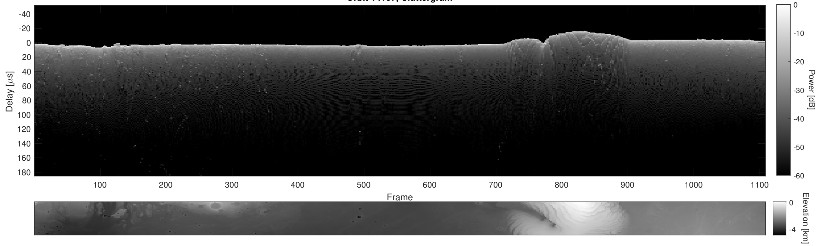
Orbit 14107, Cluttergram
