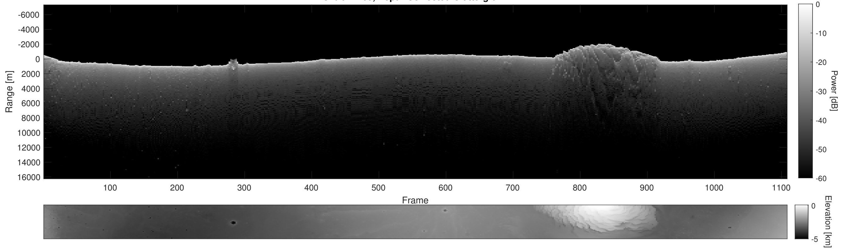
Orbit 14109, Depth-Corrected Cluttergram
