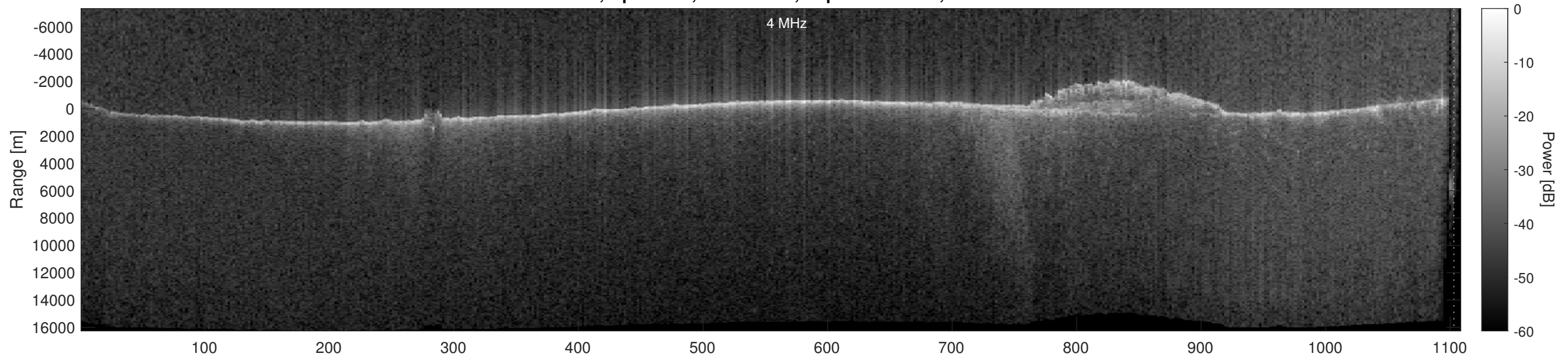
Orbit 14109, Optimized, No Window, Depth-Corrected, Channel 2
