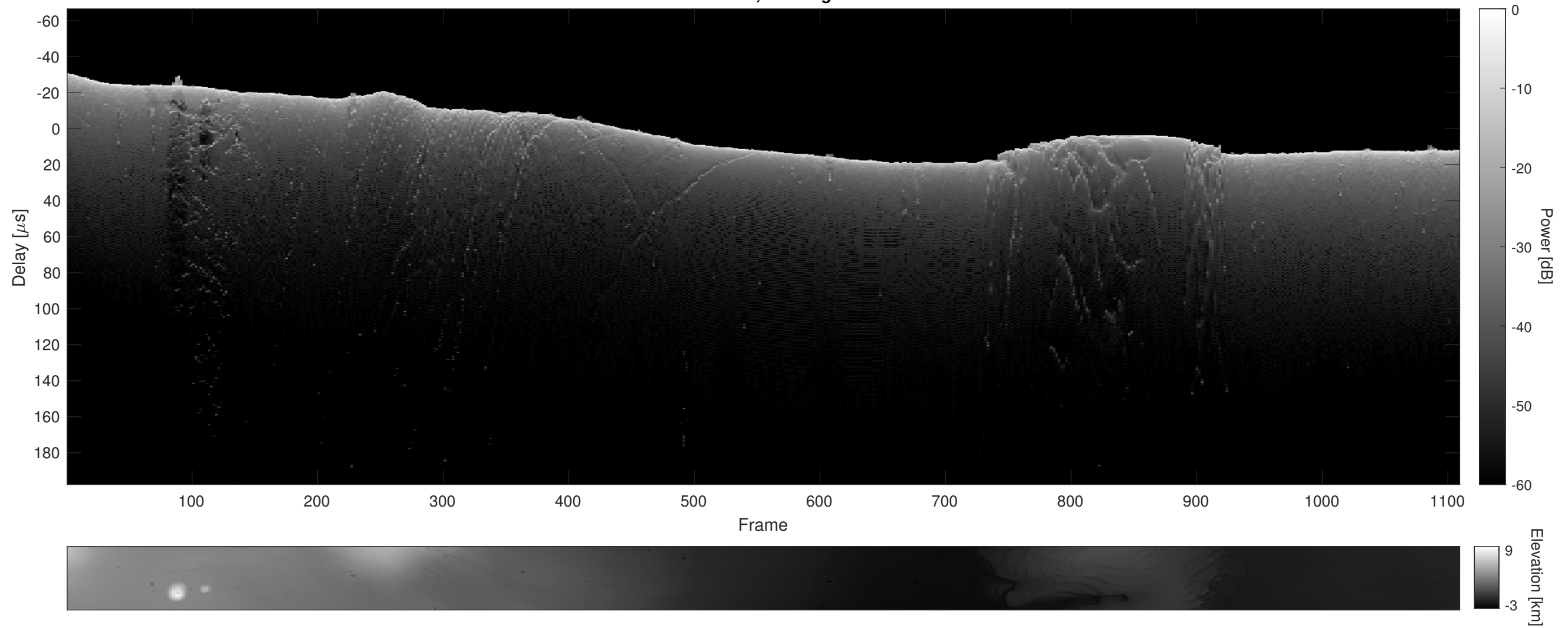
Orbit 14111, Cluttergram
