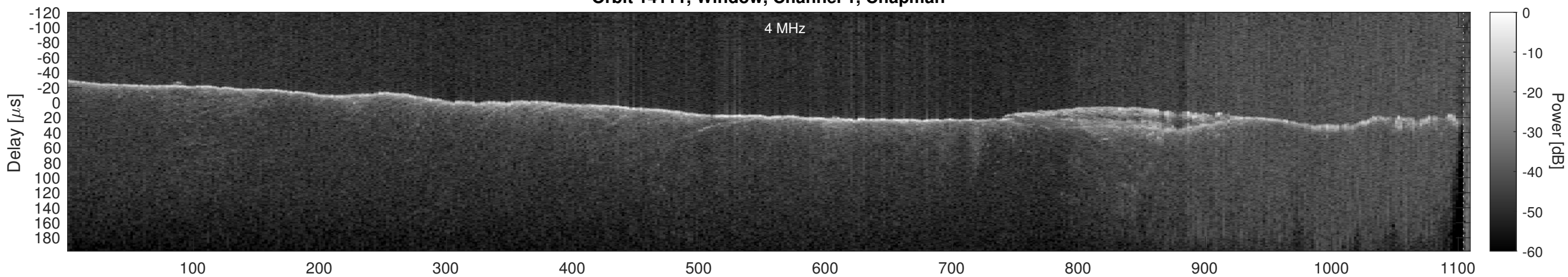
Orbit 14111, Window, Channel 1, Optimized
