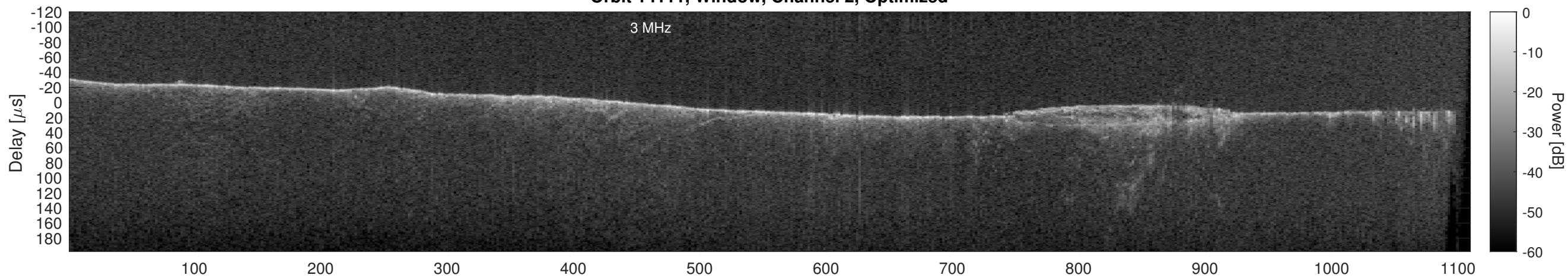
Orbit 14111, Cluttergram
