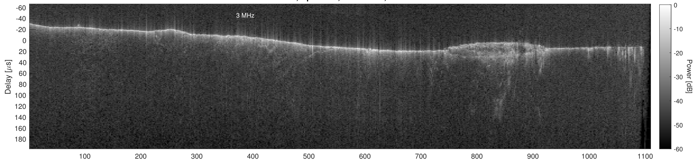
Orbit 14111, Cluttergram
