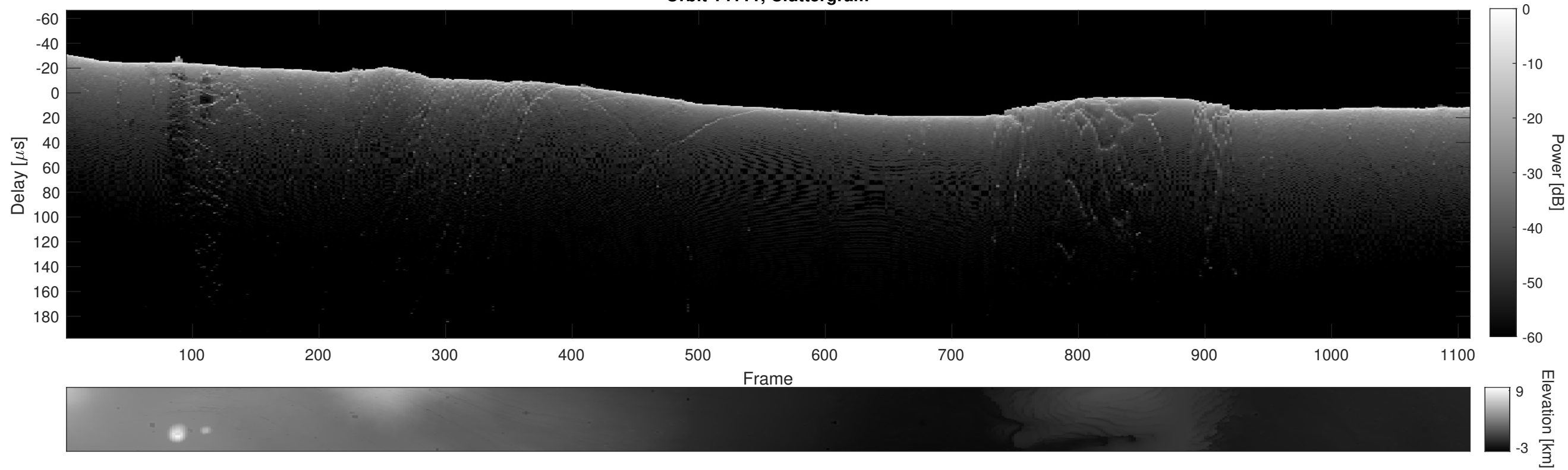
Orbit 14111, Cluttergram
