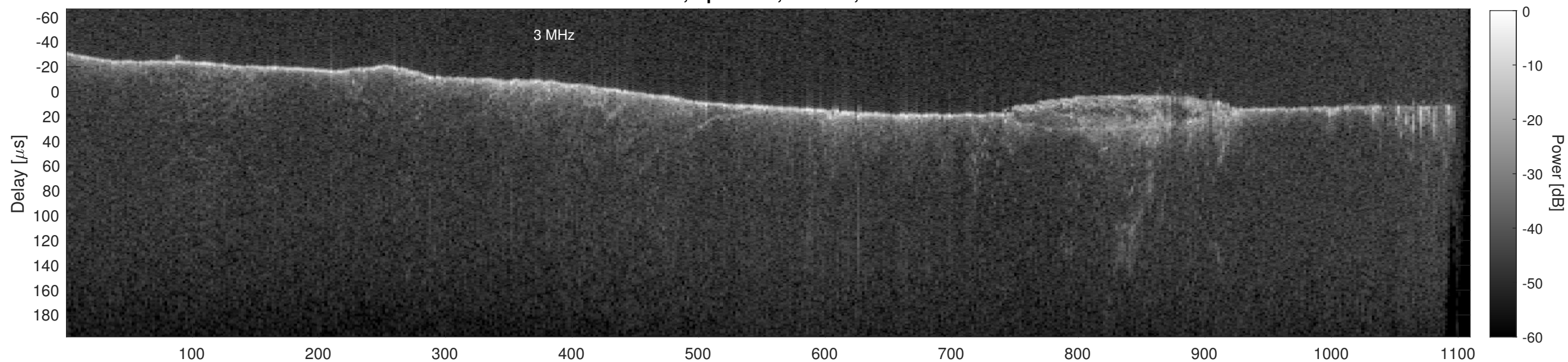
Orbit 14111, Cluttergram
