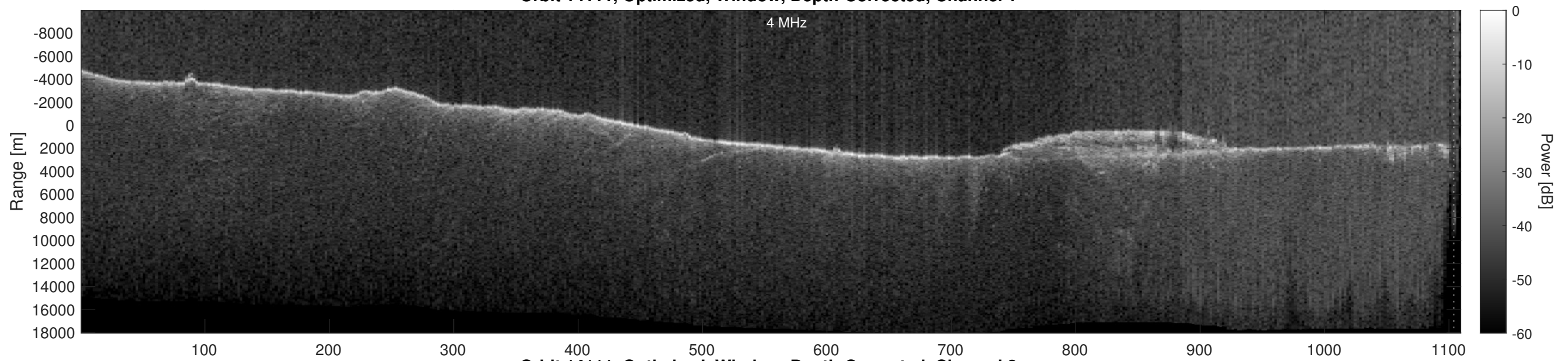
Orbit 14111, Optimized, Window, Depth-Corrected, Channel 2
