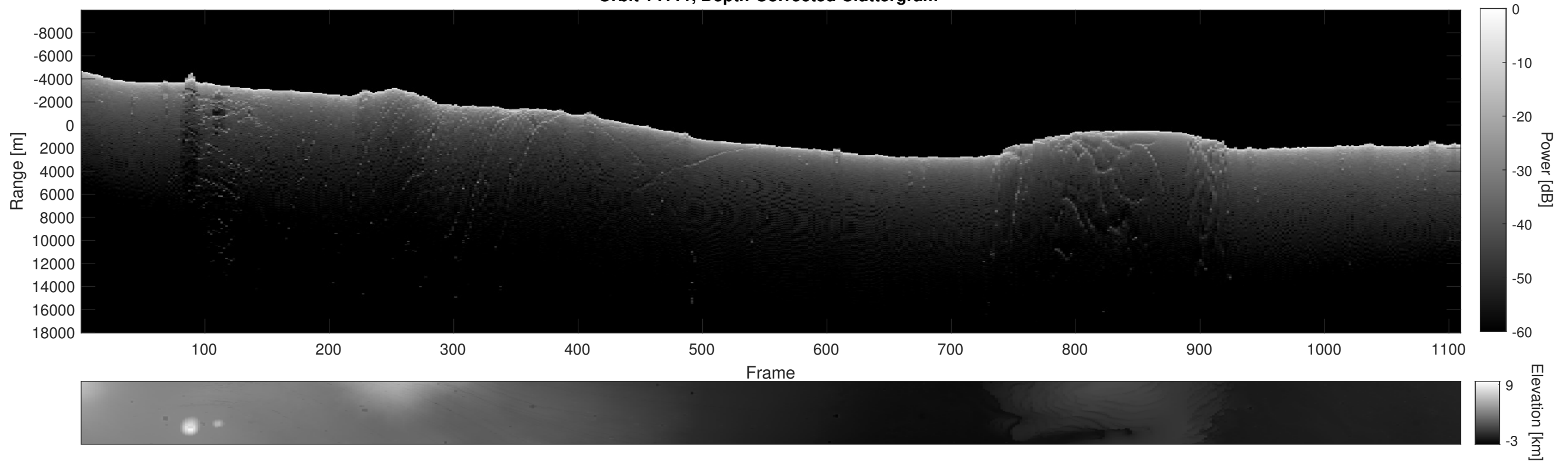
Orbit 14111, Depth-Corrected Cluttergram
