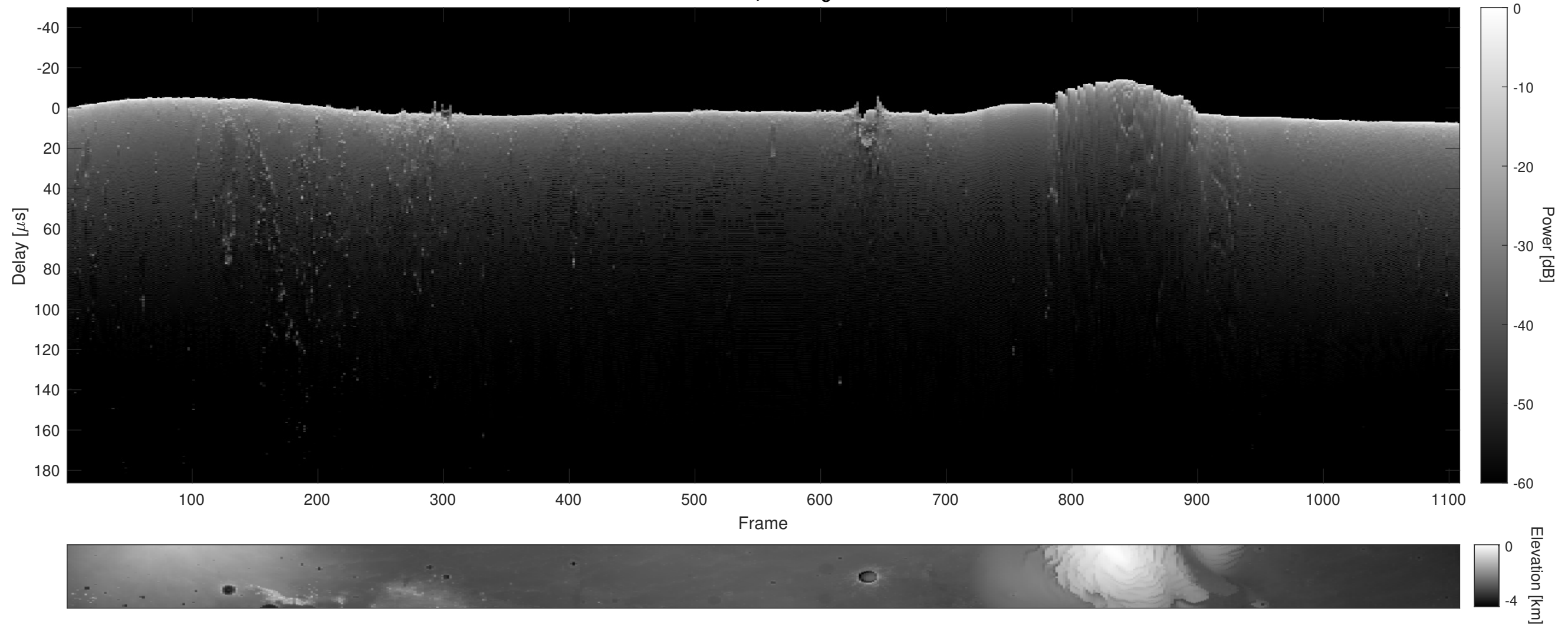
Orbit 14112, Cluttergram
