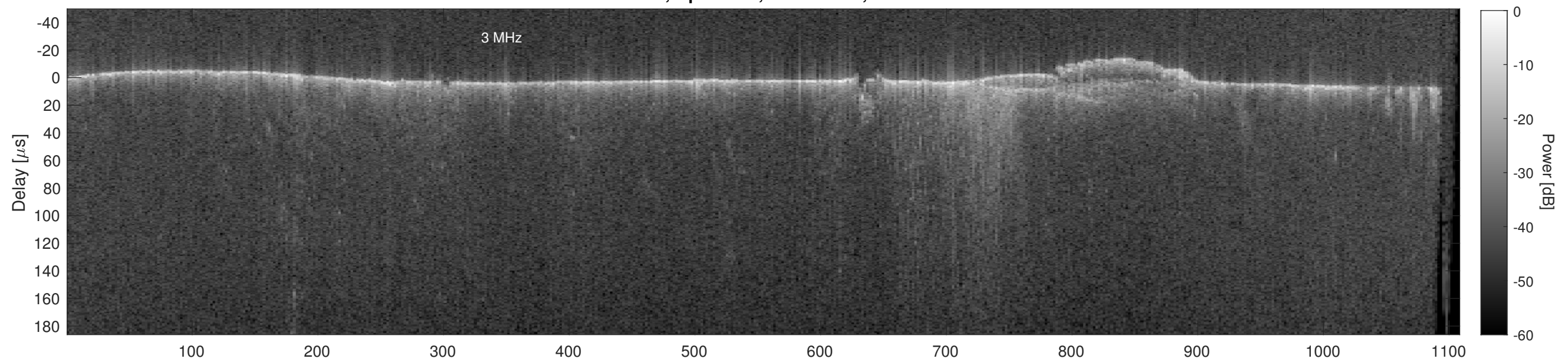
Orbit 14112, Cluttergram
