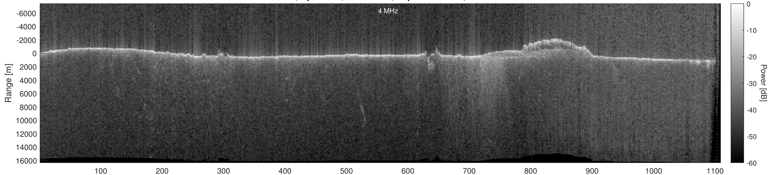
Orbit 14112, Optimized, No Window, Depth-Corrected, Channel 2
