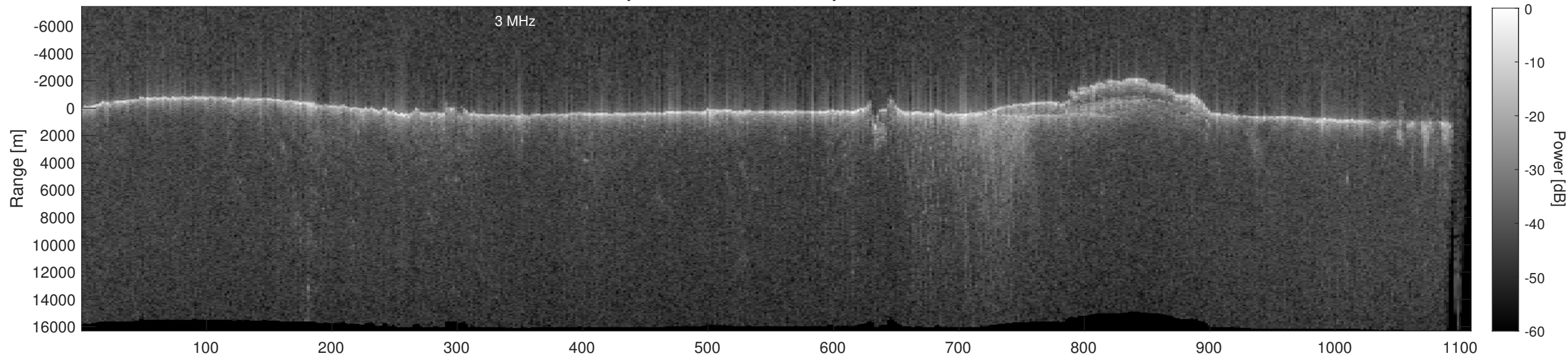
Orbit 14112, Depth-Corrected Cluttergram
