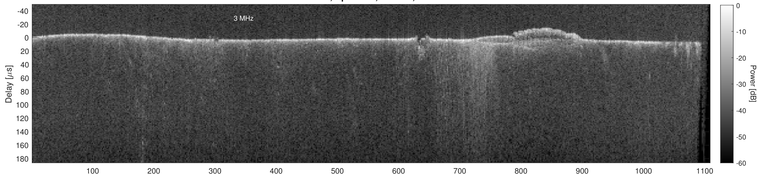
Orbit 14112, Cluttergram
