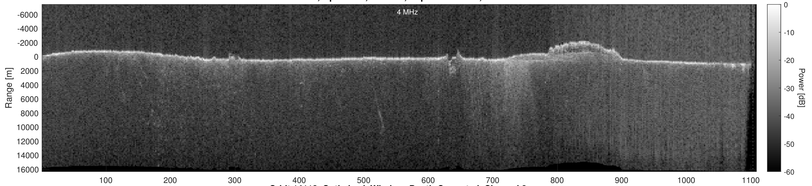
Orbit 14112, Optimized, Window, Depth-Corrected, Channel 2
