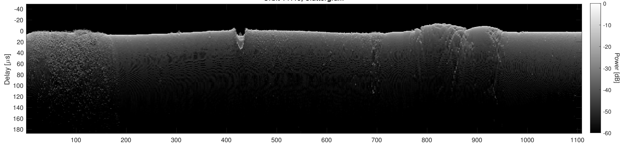
Orbit 14115, Cluttergram
