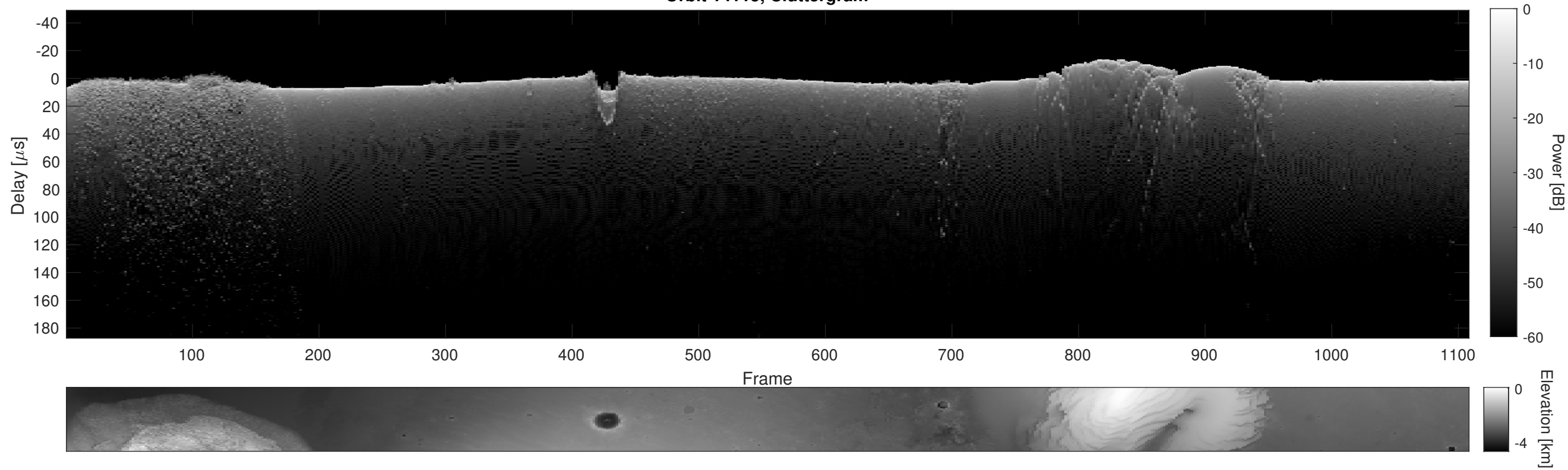
Orbit 14115, Cluttergram
