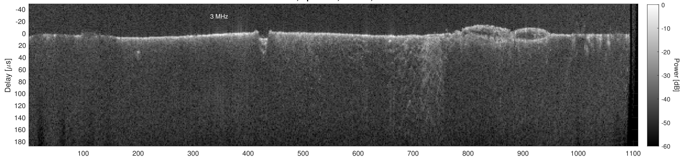
Orbit 14115, Cluttergram
