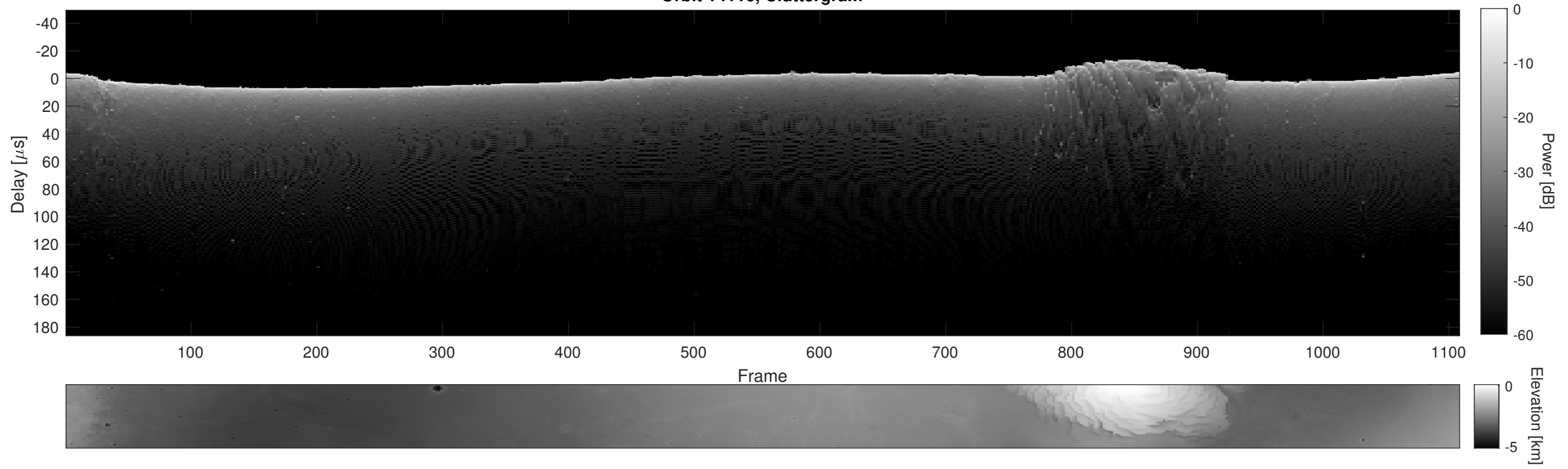
Orbit 14116, Cluttergram
