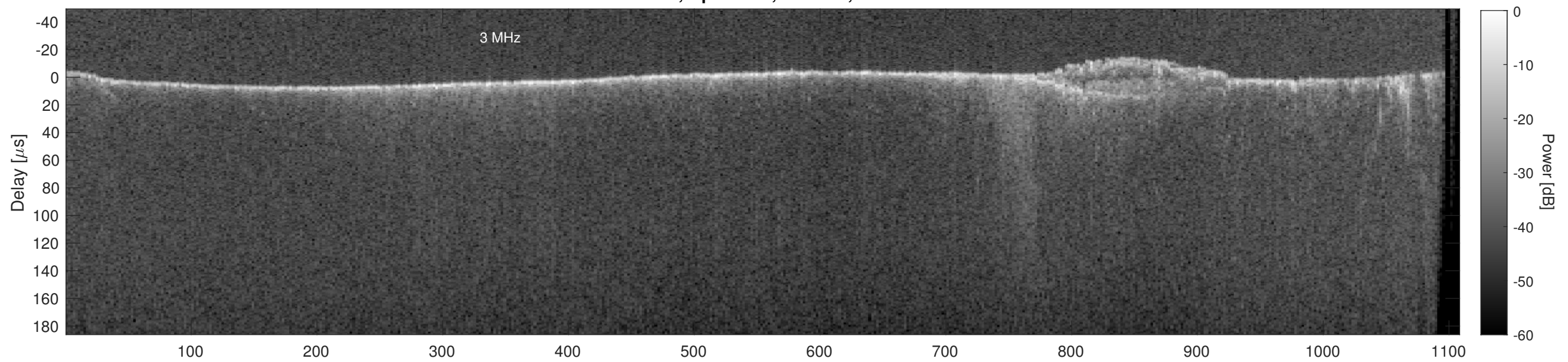
Orbit 14116, Cluttergram
