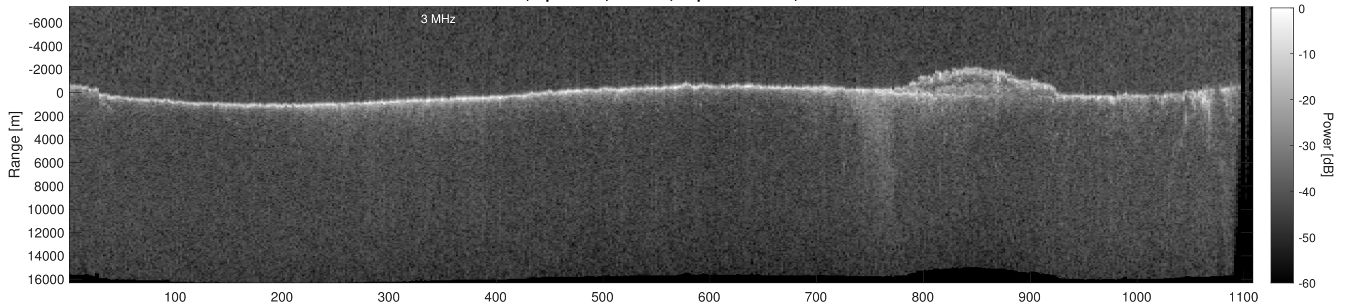
Orbit 14116, Depth-Corrected Cluttergram
