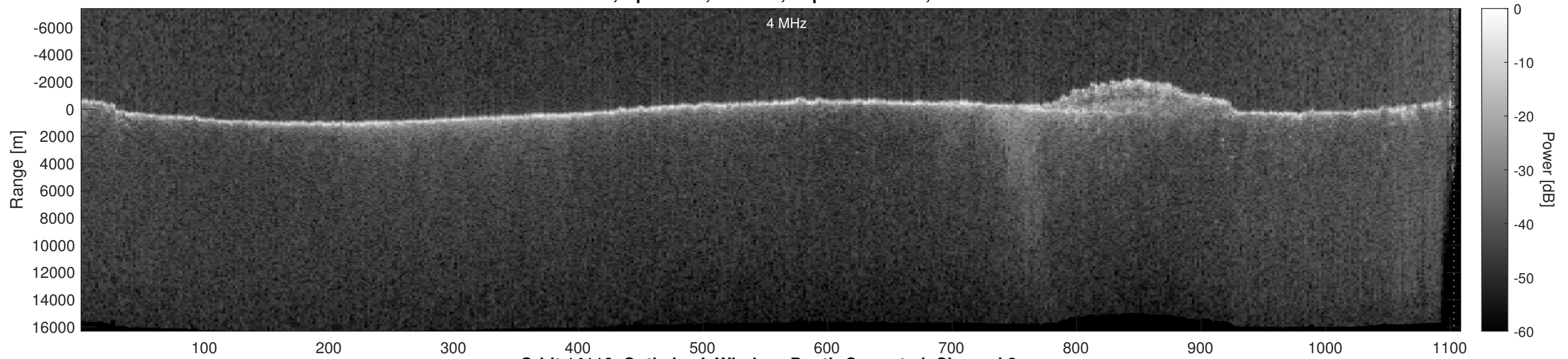
Orbit 14116, Optimized, Window, Depth-Corrected, Channel 2
