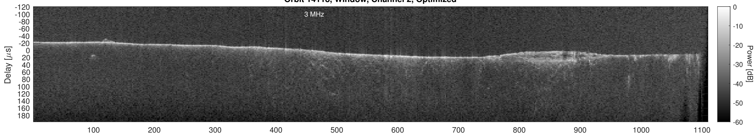
Orbit 14118, Cluttergram
