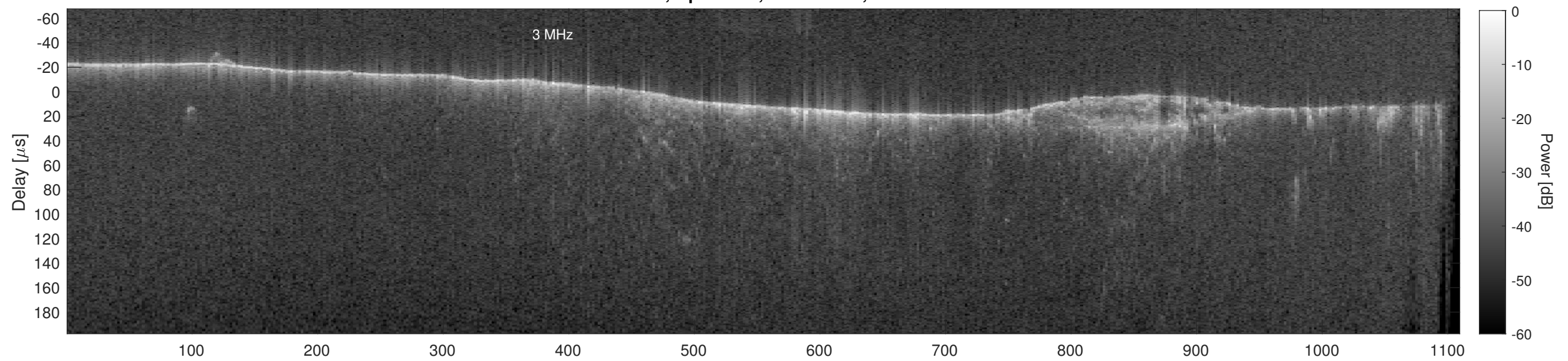
Orbit 14118, Cluttergram
