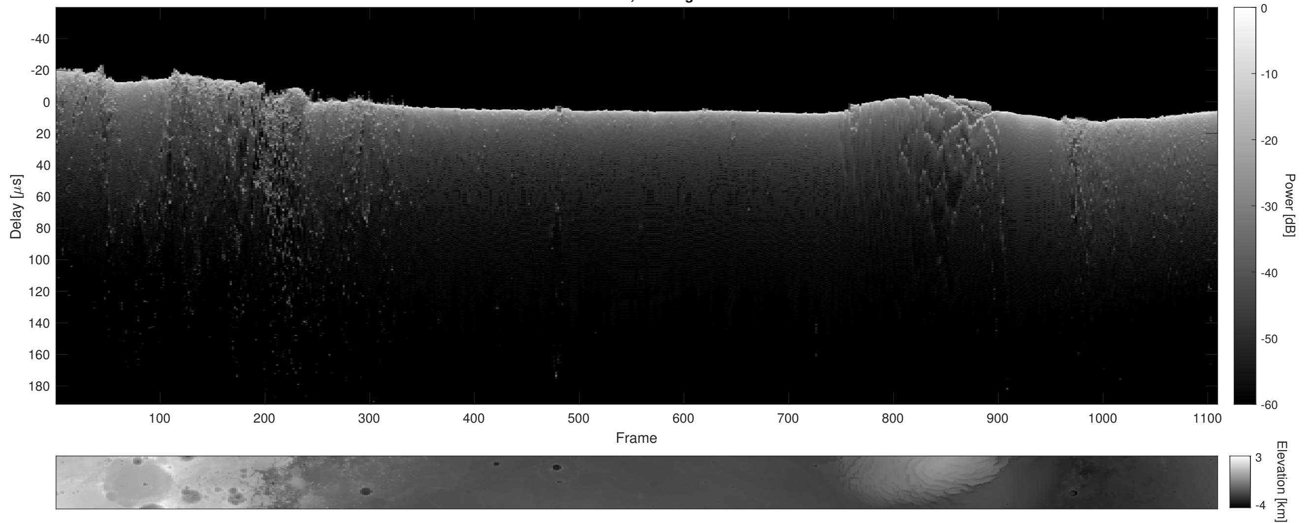
Orbit 14120, Cluttergram
