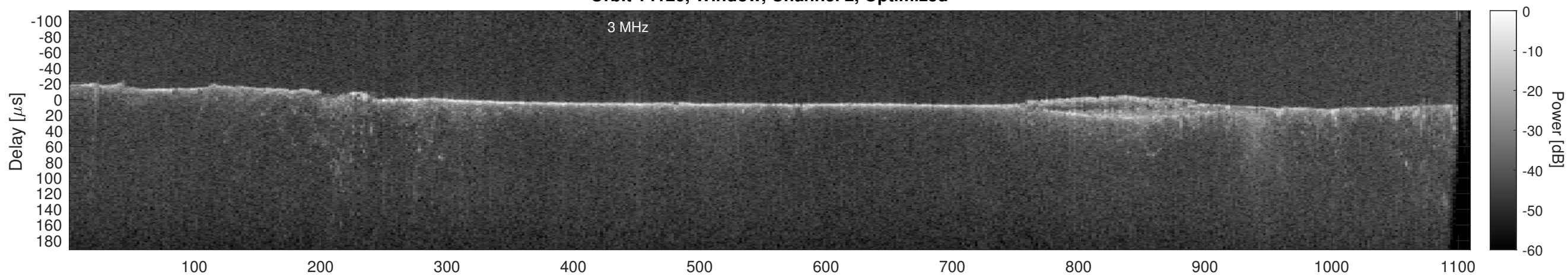
Orbit 14120, Cluttergram
