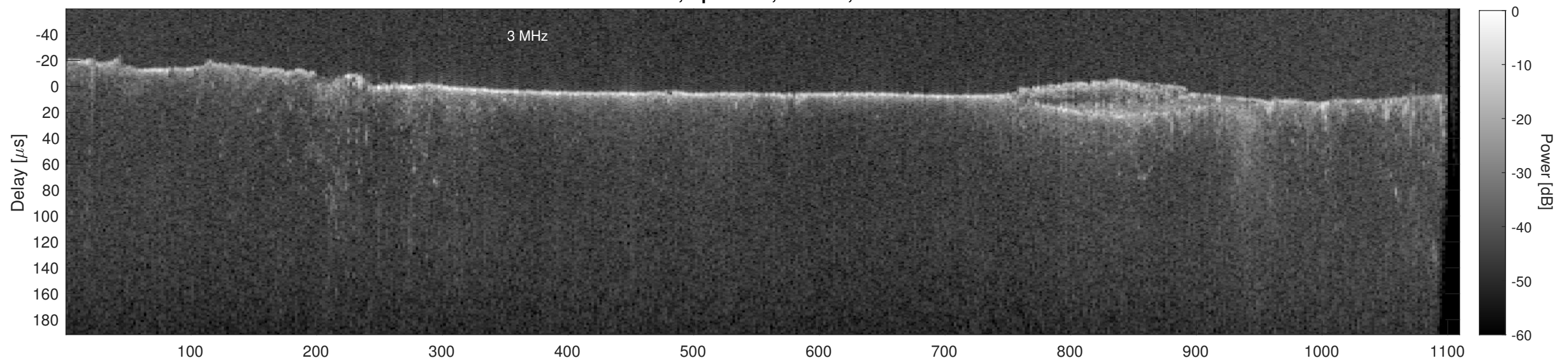
Orbit 14120, Cluttergram
