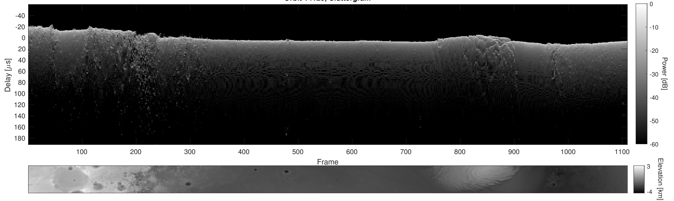
Orbit 14120, Cluttergram
