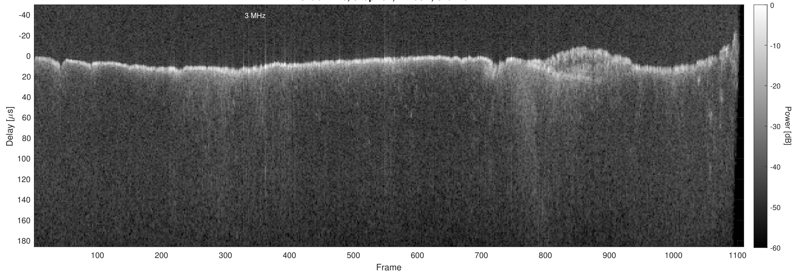
Orbit 14123, Chapman, Window, Channel 2
