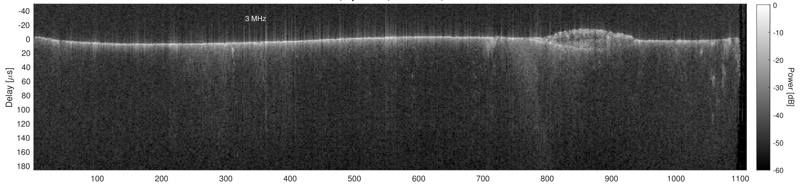
Orbit 14123, Cluttergram
