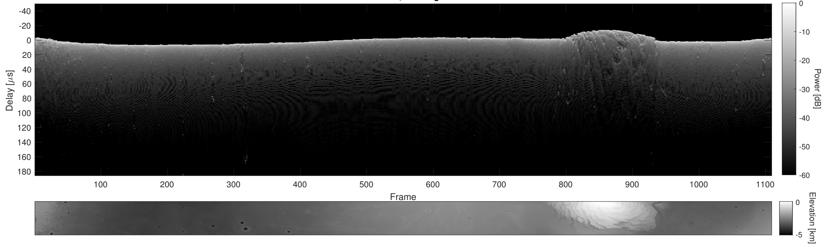
Orbit 14123, Cluttergram
