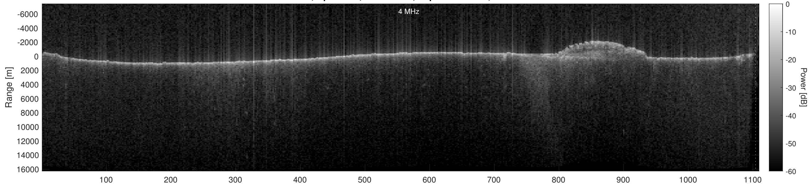
Orbit 14123, Optimized, No Window, Depth-Corrected, Channel 2
