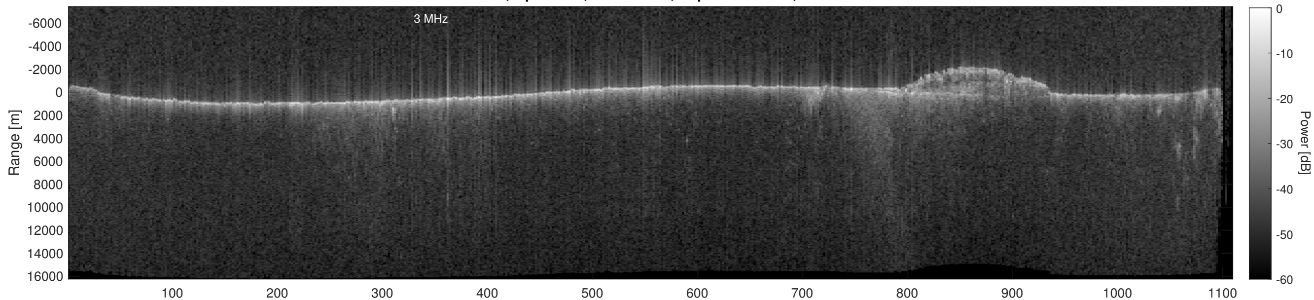
Orbit 14123, Depth-Corrected Cluttergram
