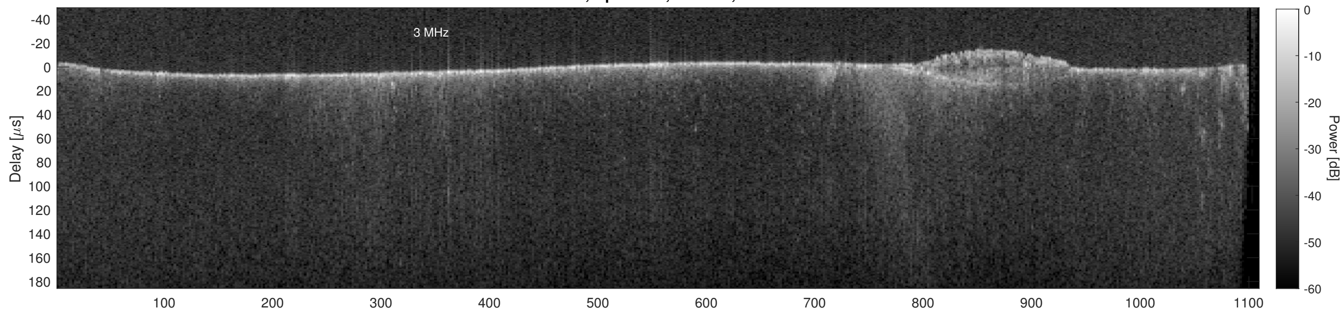
Orbit 14123, Cluttergram
