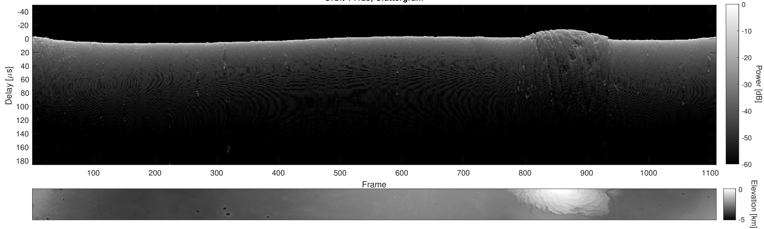
Orbit 14123, Cluttergram
