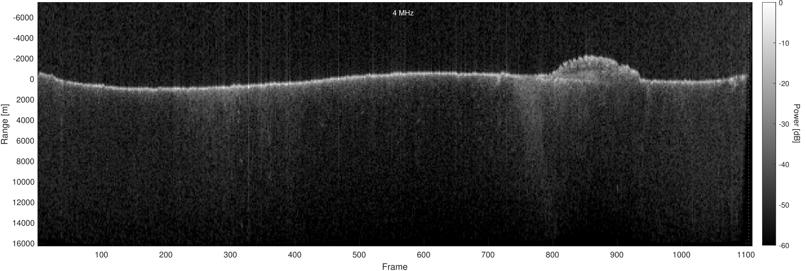
Orbit 14123, Optimized, Window, Depth-Corrected, Channel 2
