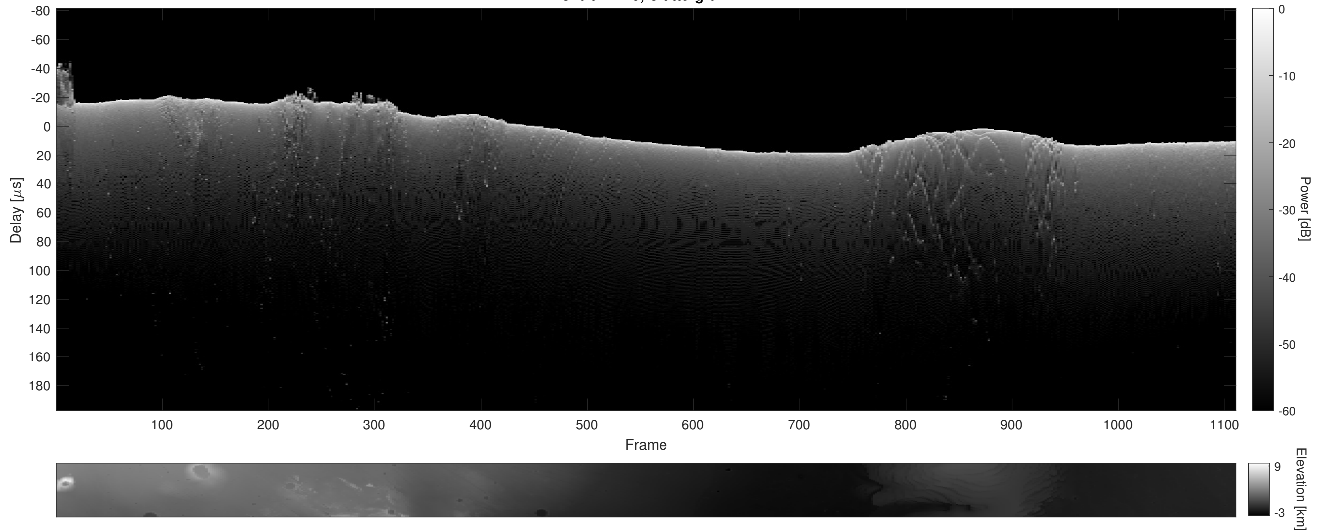
Orbit 14125, Cluttergram
