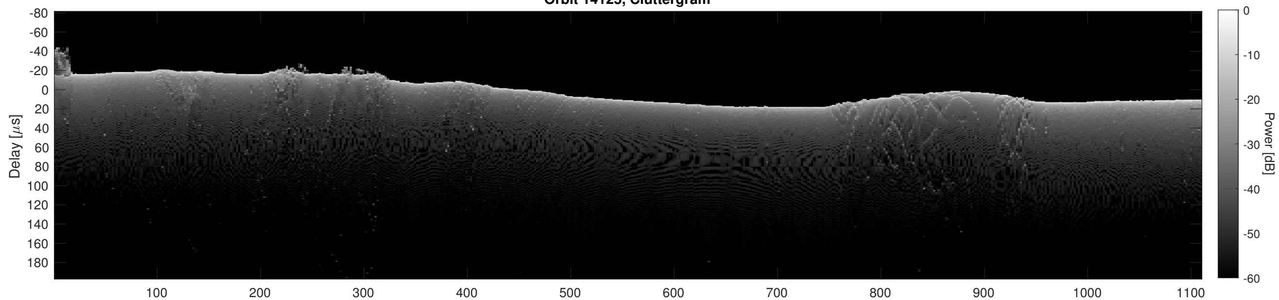
Orbit 14125, Cluttergram
