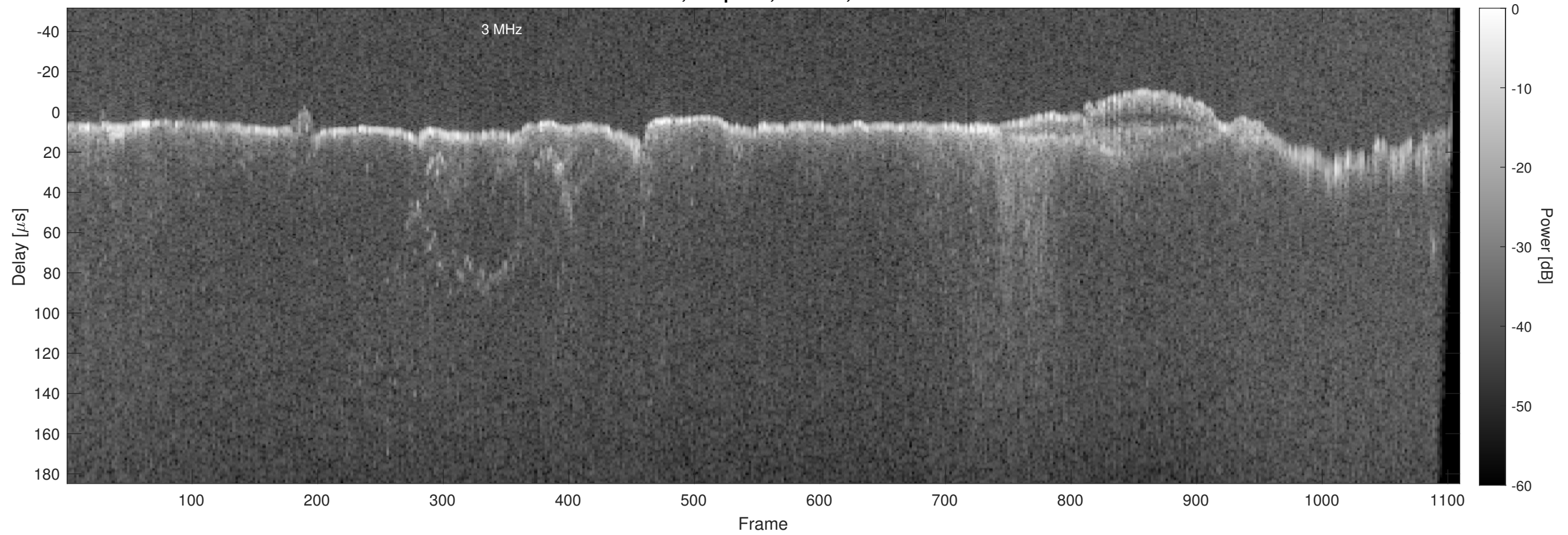
Orbit 14126, Chapman, Window, Channel 2
