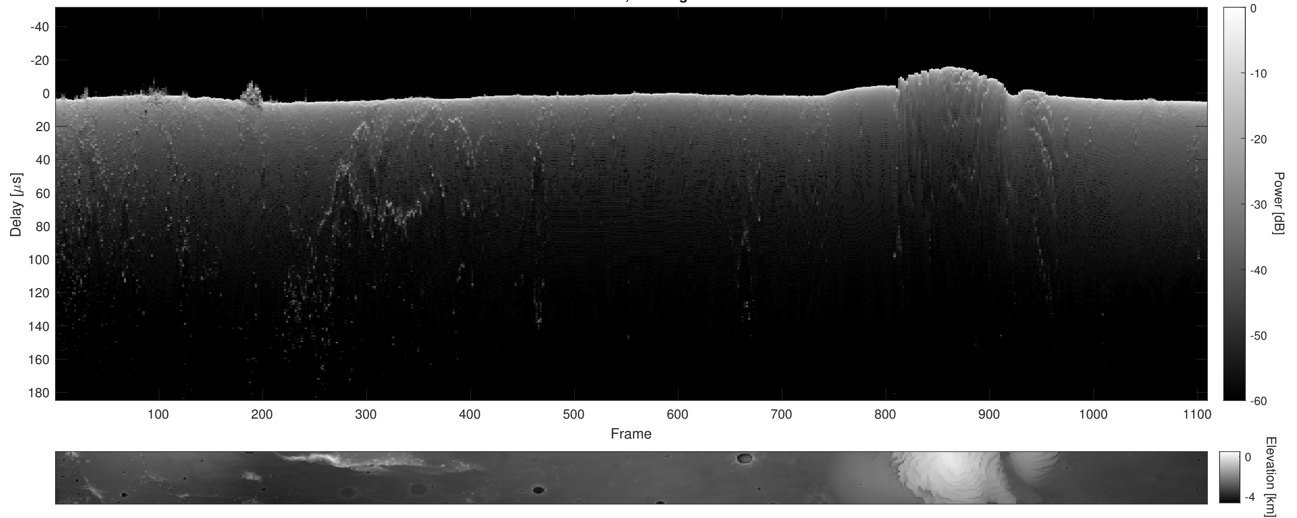
Orbit 14126, Cluttergram
