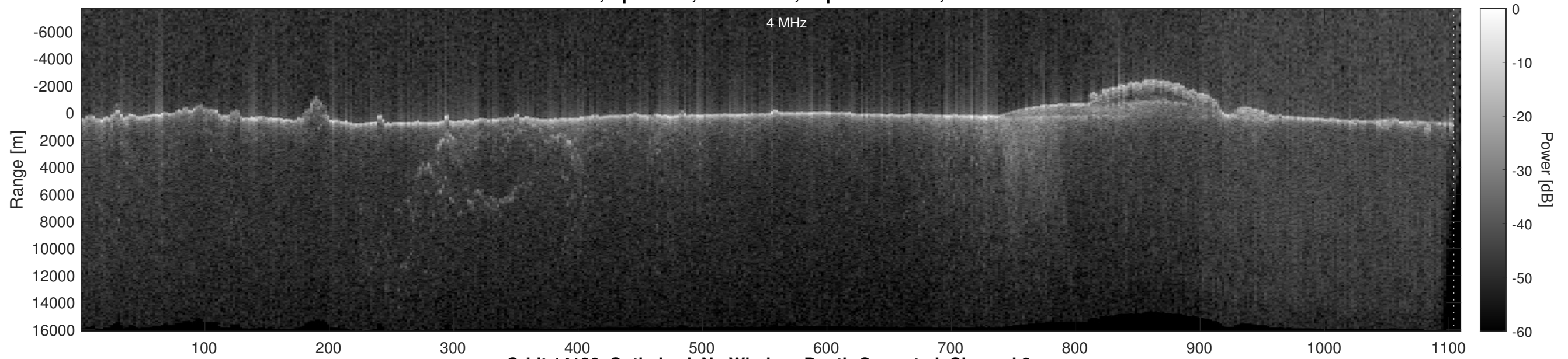
Orbit 14126, Optimized, No Window, Depth-Corrected, Channel 2
