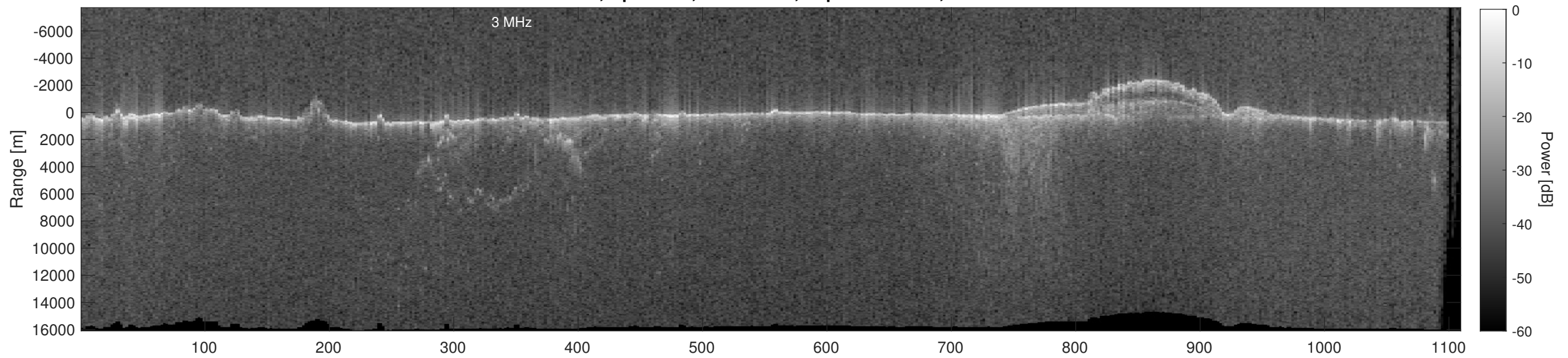
Orbit 14126, Depth-Corrected Cluttergram
